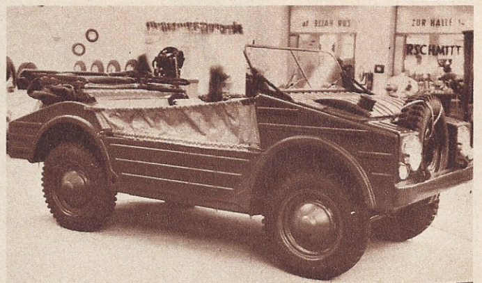
First showing of the Porsche Jeep. With a 5-speed gearbox, 4-wheel drive, and a weight of only 1900 lbs., it will top 75 mph on the road and float like a duck in the water.
